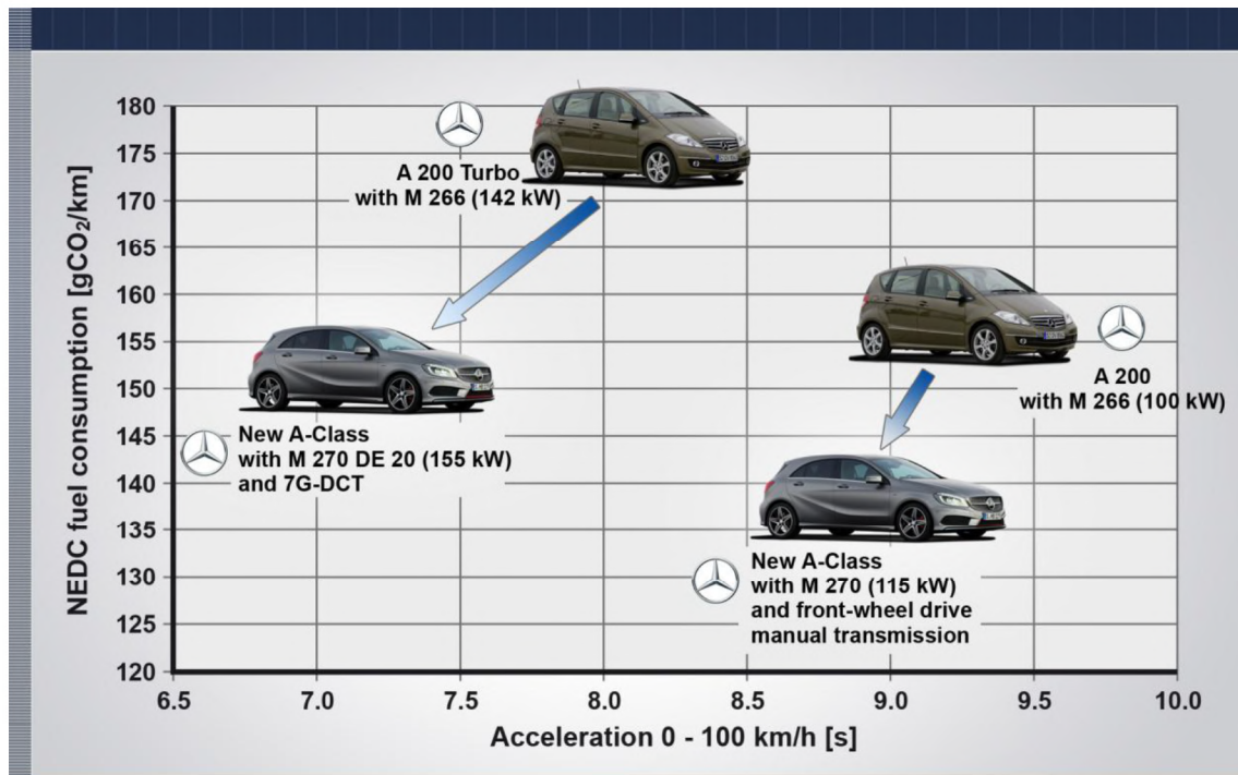
Figure 10: Driving performance comparison with the predecessor model
