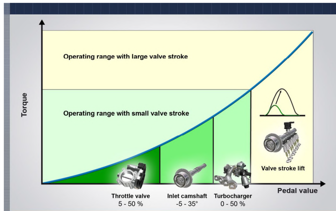
Figure 8: Camtronic operating modes on the characteristics map
