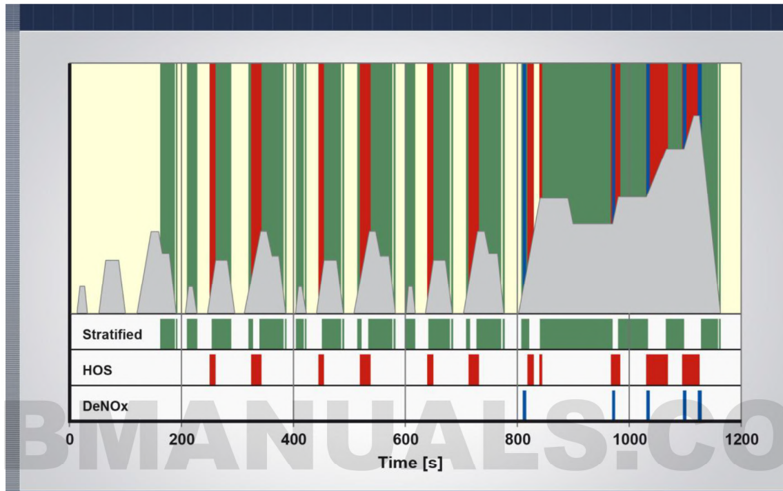
Figure 16: Vehicle operation strategy in the NEDC
