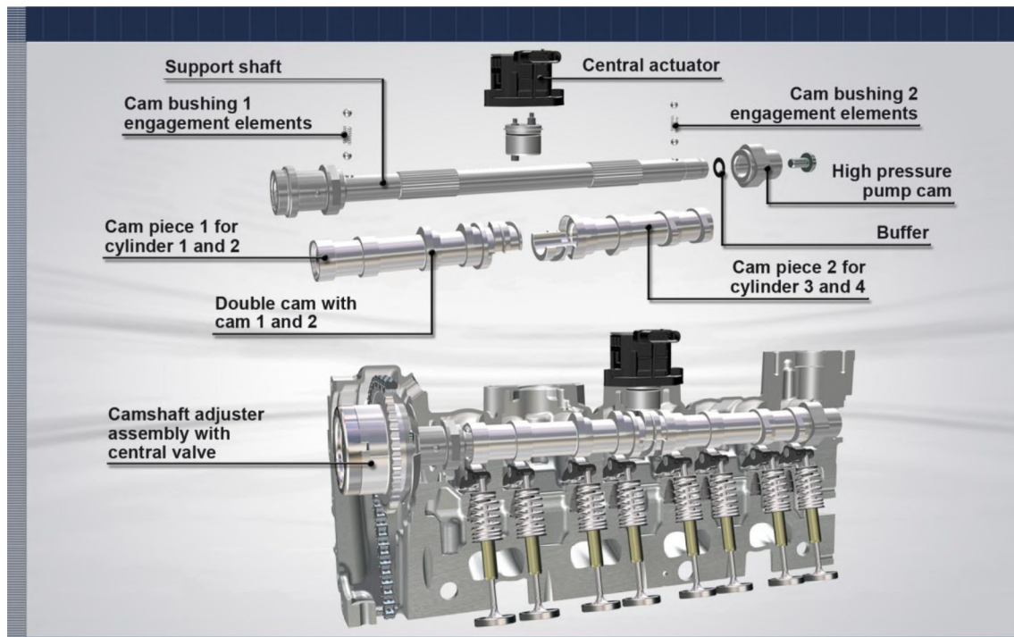
Figure 4: Camtronic layout
