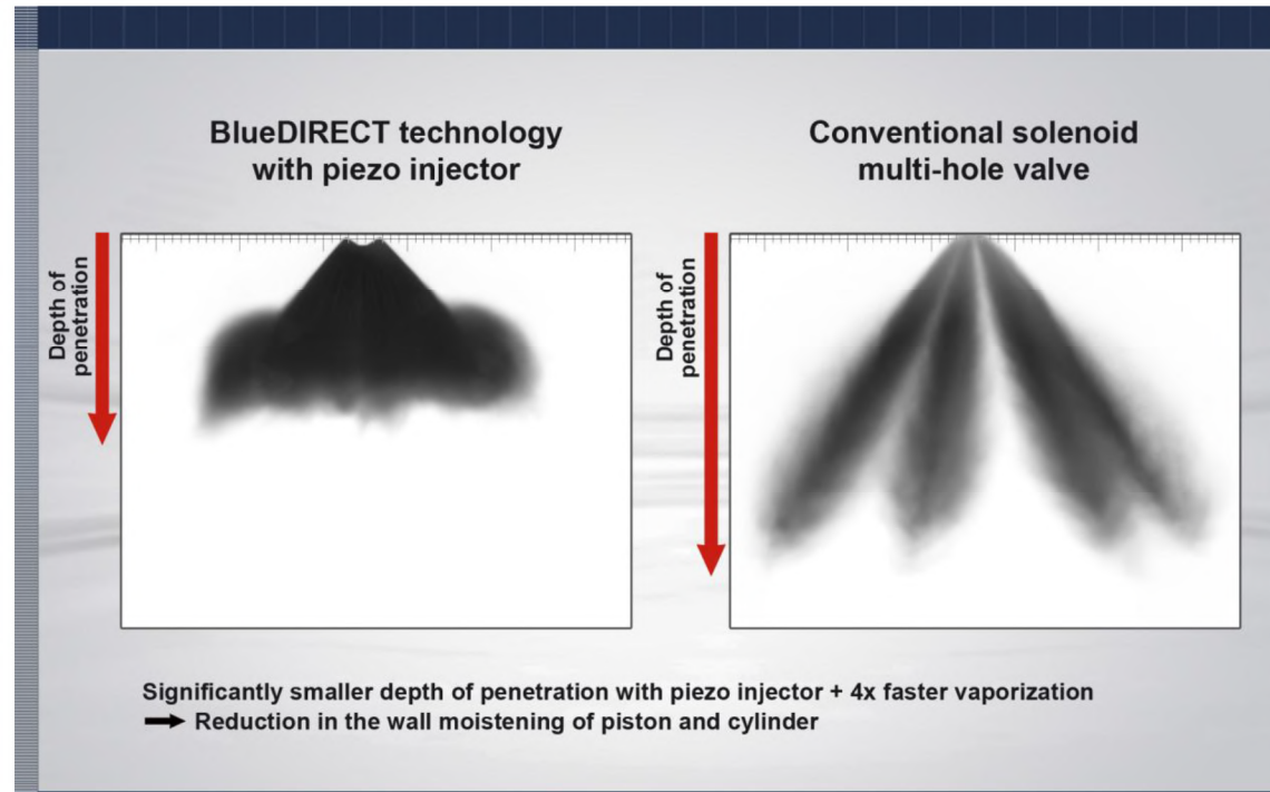
Figure 13: Comparison of injector technologies
