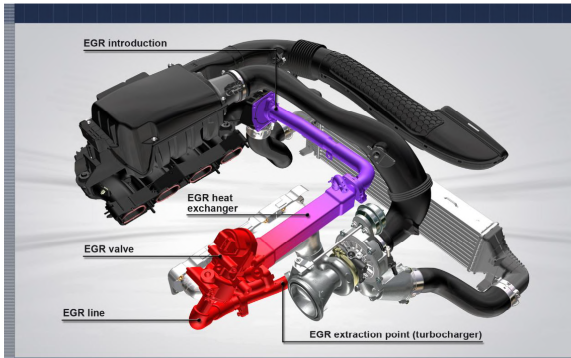
Figure 12: EGR system of the stratified engine
