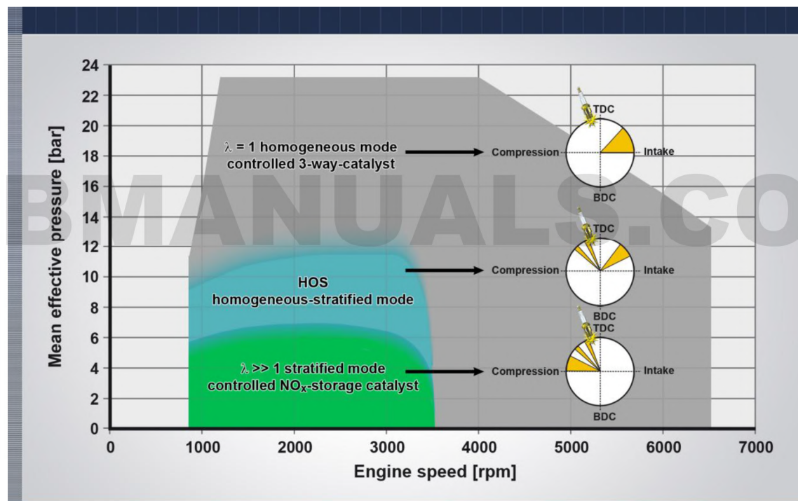
Figure 14: Operation strategies on the characteristics map
