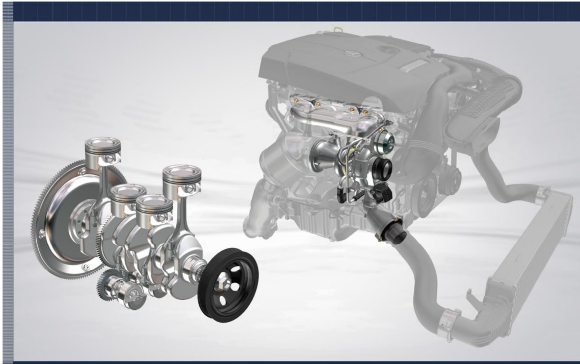
Figure 9: Change scope for 2.0l M274/270 engine
